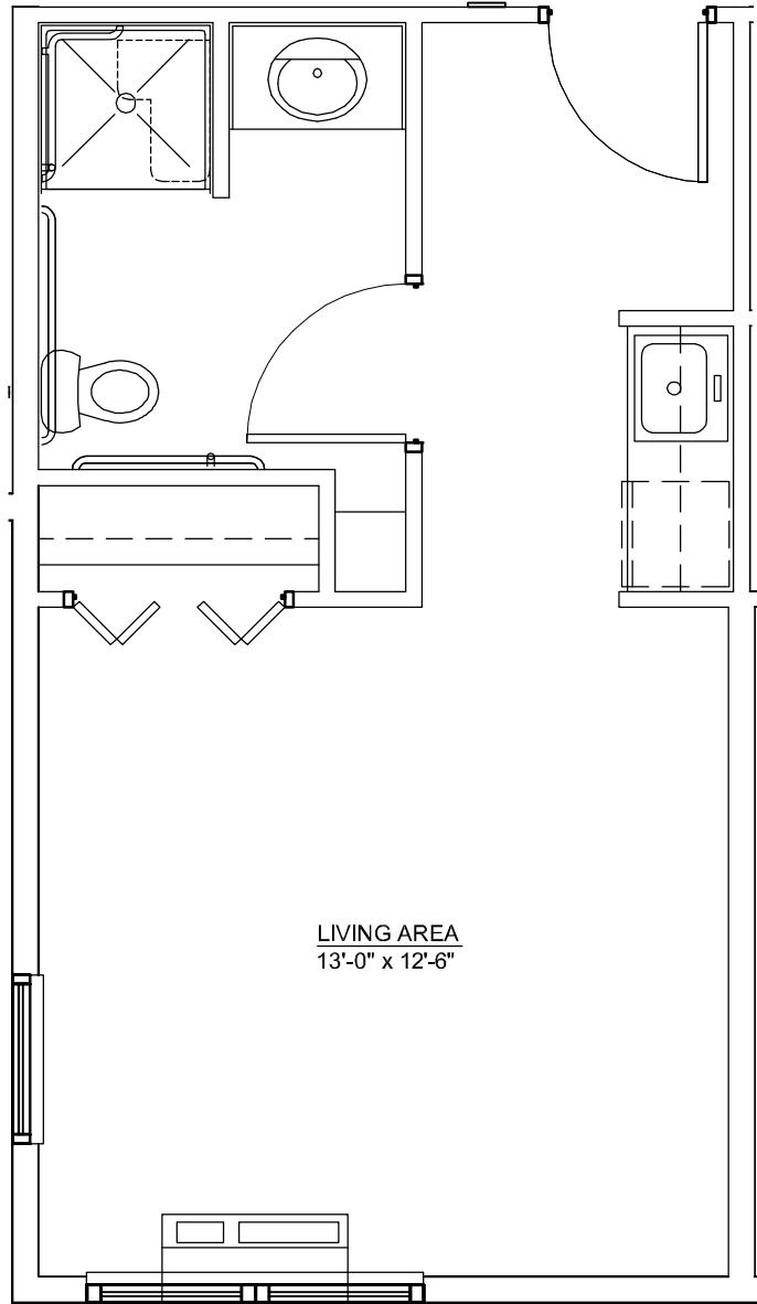
UNIT "A" (MODIFIED) PLAN
